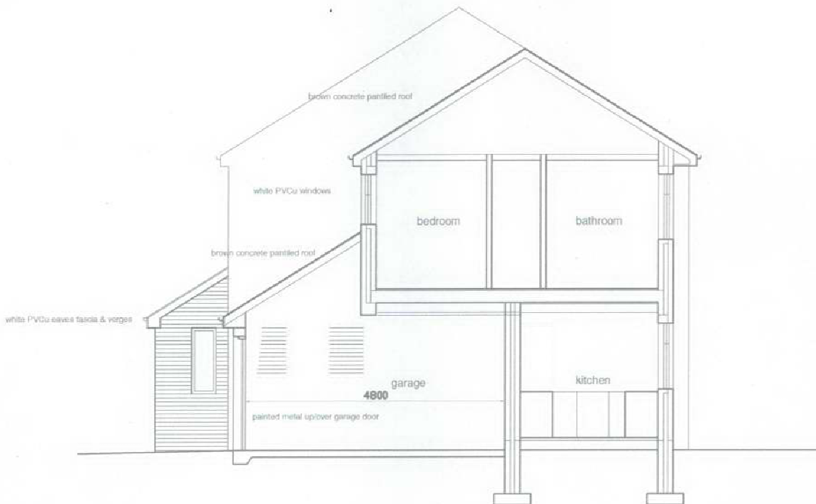
Cross Section A - A ( proposed )
